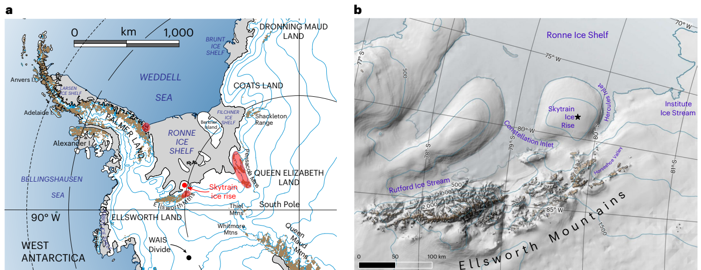
Fig. 1 | Map of SIR ice core drilling site ( 79^{\circ}44.46'S , 78^{\circ}32.69'W ). a, b , Regional map 48 based on USGS Antarctic Overview map (a) and local map of the SIR developed using the Quantarctica mapping environment detailed in Matsuoka et al. (2021) 49 (b). a , The red shading shows the locations 9,15,42–44 of the cosmogenic
